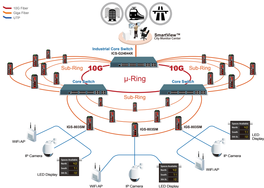
Figure 2 : 10G Backbone with μ-Ring topology
